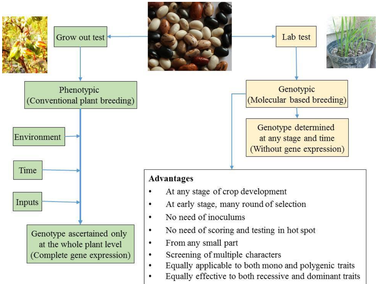
Figure 11. Comparative process and advantages between grow out test and lab test in selection or identification of genotype
