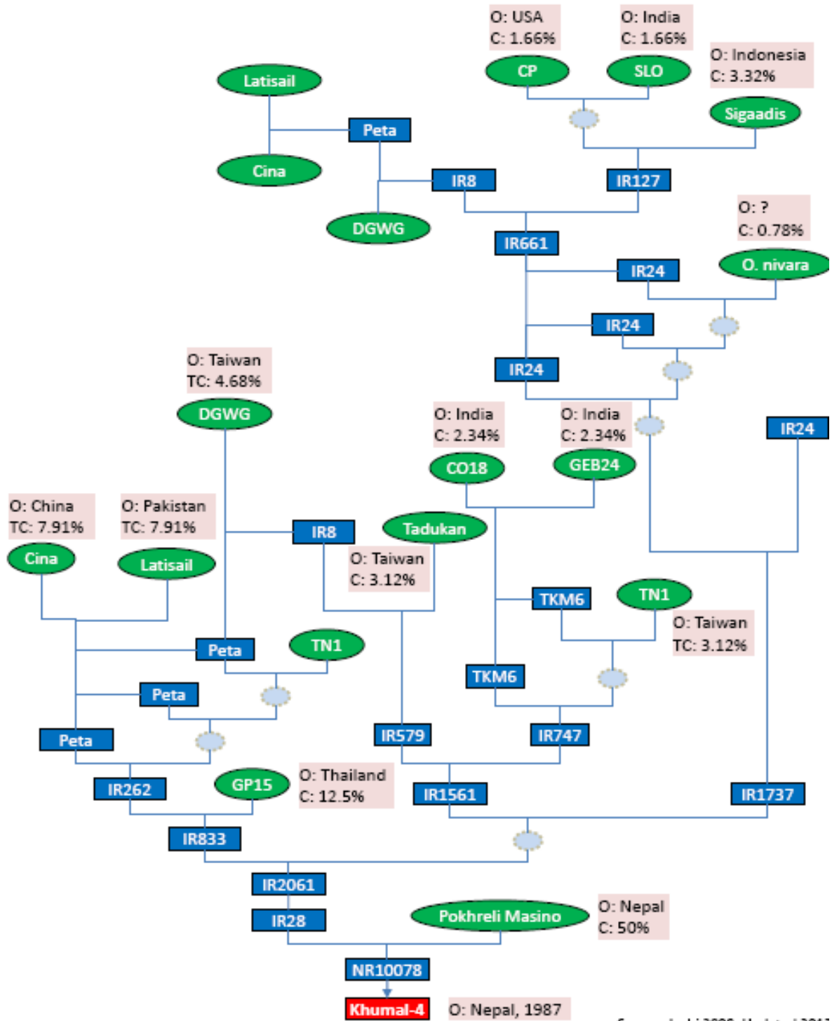
Figure 5. Complete pedigree tree and ancestral contribution to Khumla-4 rice variety
